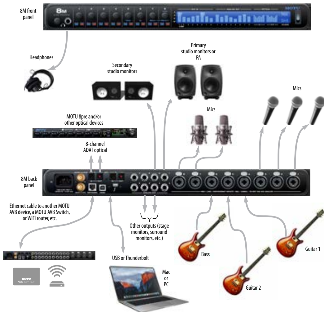
Figure 4-14: A typical 8M studio setup.
