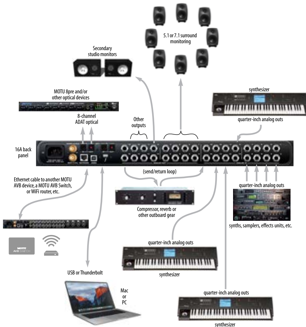
Figure 4-15: A typical 16A studio setup.
