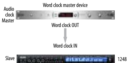
Figure 4-21: Slaving your MOTU device (a 1248 in this example) to word clock. For the 1248 clock source, choose 'Word Clock In'.
