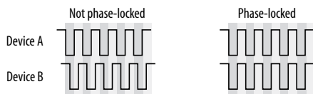
Figure 4-18: When transferring audio, two devices must have phase-locked audio clocks to prevent clicks, pops or other artifacts.
