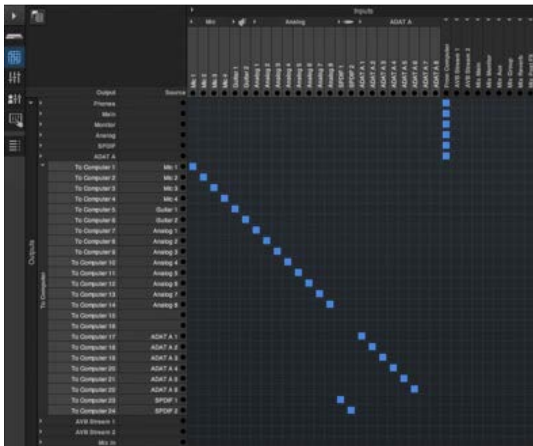
Figure 7-7: An example of routing physical inputs on the 1248 to computer channels (for host audio software). In this example, S/PDIF input is on channels 23-24 going to the computer, and 24 channels total are being used for streaming to the host computer, but more can be added for other inputs from the mixer or AVB network, if any.
