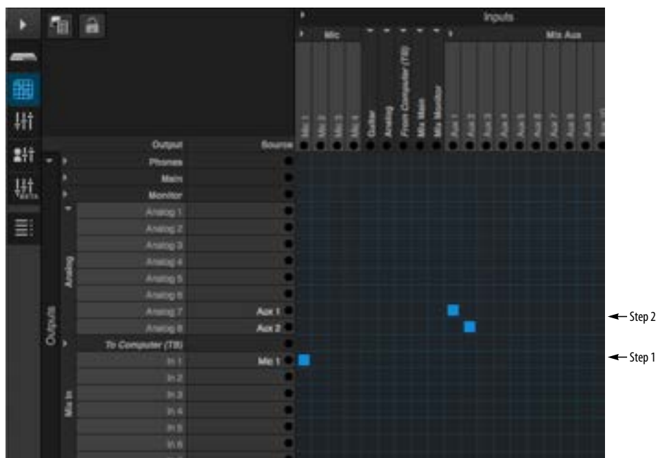
Figure 4-16: Basic routing for the built-in talkback mic. In this example, the talkback mic is connected to mic input 1, which is routed to input 1 of the mixer. Aux bus 1-2 is assigned to analog outs 7-8, which are being used to route the signal to speakers in the room where the musicians are located.
